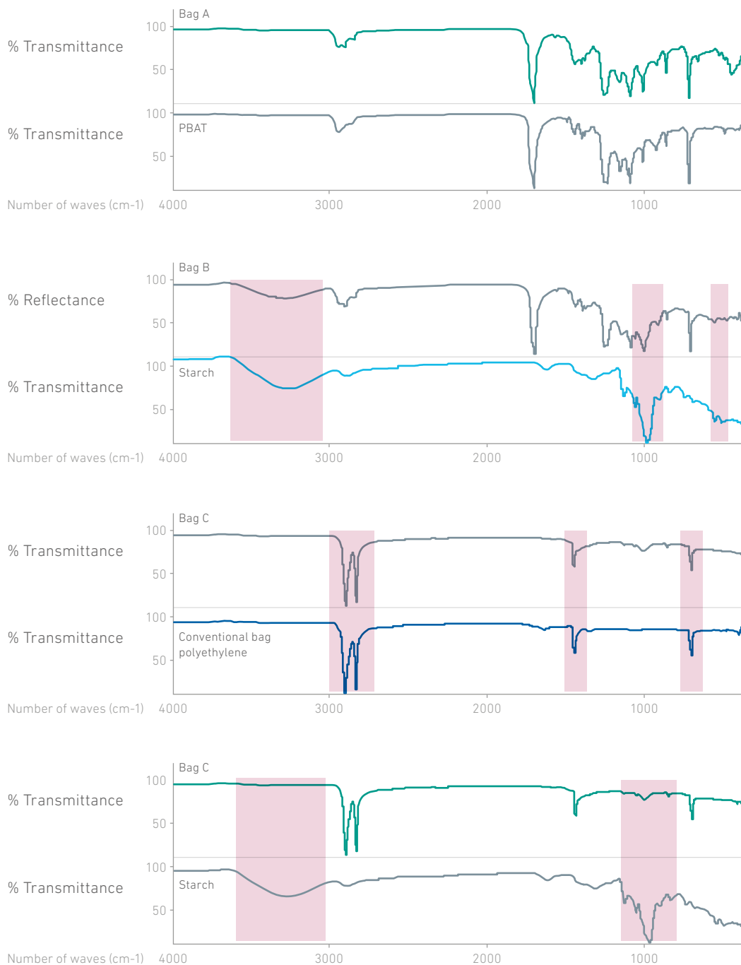
Figure 2. Identification of polymeric compounds by infrared spectroscopy
